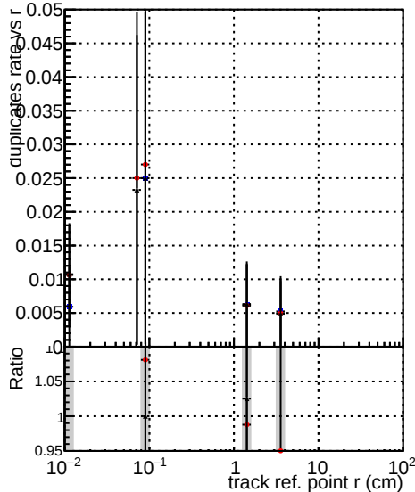
—●— DQM_V0001_R000000001 Global mkFit_baseline —●— DQM_V0001_R000000001 Global mkFit_core50maxCand-24DUPremoval-1000 —●— DQM_V0001_R000000001 Global mkFit_core10maxCand-24DUPremoval-1000
