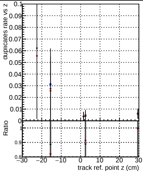
—●— DQM_V0001_R000000001 Global mkFit_baseline —●— DQM_V0001_R000000001 Global mkFit_core50maxCand-24DUPremoval-1000 —●— DQM_V0001_R000000001 Global mkFit_core10maxCand-24DUPremoval-1000
