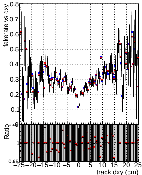
DOM V0001 R0000000001 Global mkFit baseline DOM V0001 R0000000001 Global mkFit [core50maxCand-24DUPremoval-1000] DOM V0001 R0000000001 Global mkFit [core10maxCand-24DUPremoval-1000]
