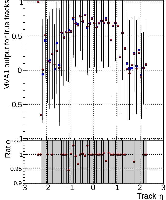
MVA1 of associated tracks (recoToSim) vs. track \eta Legend: Global mkFit baseline (blue squares) Global mkFit jcore50maxCand-24DUPremoval-1000 (red circles) Global mkFit jcore10maxCand-24DUPremoval-1000 (black triangles)
