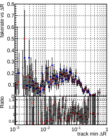
Legend: —●— DQM_V0001_R0000000001_Global_mkFit_baseline —●— DQM_V0001_R0000000001_Global_mkFit_core50maxCand-24DUPremoval-1000 —●— DQM_V0001_R0000000001_Global_mkFit_core10maxCand-24DUPremoval-1000
