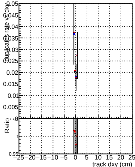
Legend for all plots: DOM V0001 R0000000001 Global mkFit baseline DOM V0001 R0000000001 Global mkFit [core10maxCand-24DUPremoval-1000] DOM V0001 R0000000001 Global mkFit [core10maxCand-24DUPremoval-1000]
