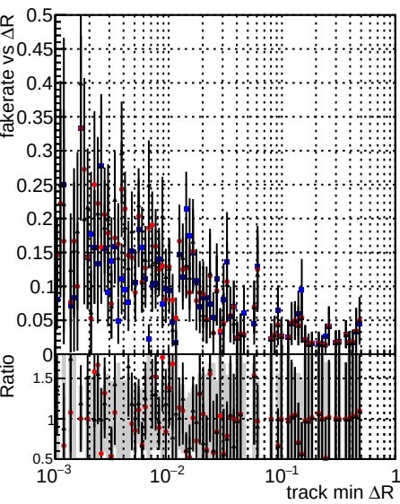
Legend: DQM_V0001_R000000001 Global mkFit baseline, DQM_V0001_R000000001 Global mkFit_jcore50maxCand-24DUPremoval-1000, DQM_V0001_R000000001 Global mkFit_jcore10maxCand-24DUPremoval-1000
