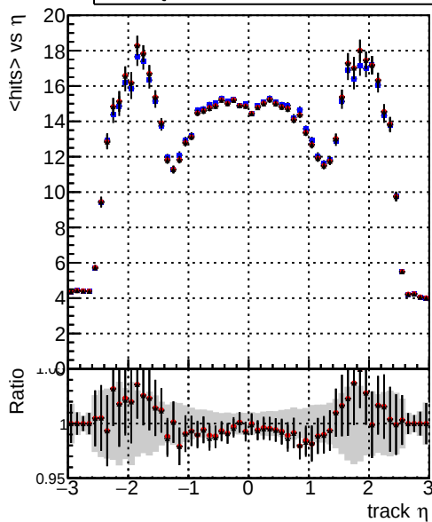
mean hits vs \eta — DQM_V0001_R000000001_Global_mkFit_baseline — DQM_V0001_R000000001_Global_mkFit_core50maxCand-24DUPremoval-1000 — DQM_V0001_R000000001_Global_mkFit_core10maxCand-24DUPremoval-1000
