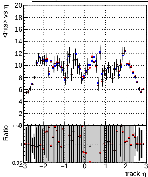
mean hits vs \eta Legend: - Blue line: DQM_V0001_R000000001_Global_mkFit_baseline - Red line: DQM_V0001_R000000001_Global_mkFit_core50maxCand-24DUPremoval-1000 - Black line: DQM_V0001_R000000001_Global_mkFit_core10maxCand-24DUPremoval-1000
