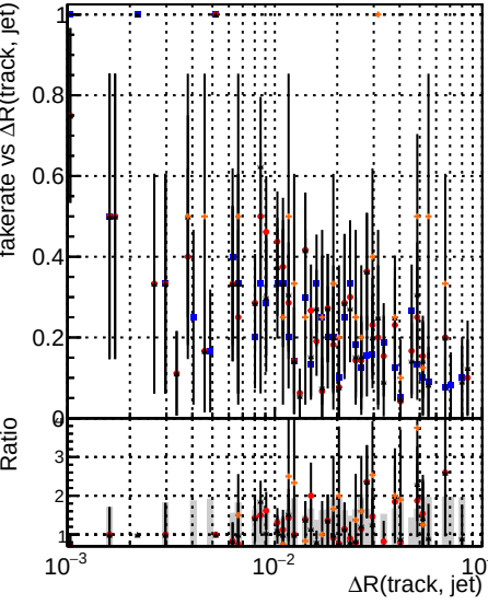
Fake rate vs \Delta R(\text{track, jet}) | Duplicates Rate vs \Delta R(\text{track, jet}) | Pileup rate vs \Delta R(\text{track, jet}) Legend: - Global mkFit baseline - Global mkFit var - Global mkFit coreNoClean - Global mkFit core50maxCand-45DUPremoval
