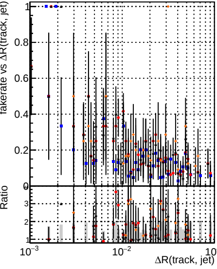
Fake rate vs \Delta R(\text{track, jet}) DQM V00001 Global mkFit baseline Global mkFit var Global mkFit coreNoClean Global mkFit core50maxCand-45DUPremoval
