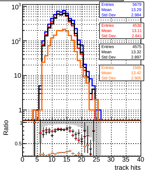
Legend: DQM_V0001_R000000001_Global_mkFit_baseline (blue line), DQM_V0001_R000000001_Global_mkFit_var (red line), DQM_V0001_R000000001_Global_mkFit_coreNoClean (black line), DQM_V0001_R000000001_Global_mkFit_icore50maxCand-45DUPremoval (orange line)
