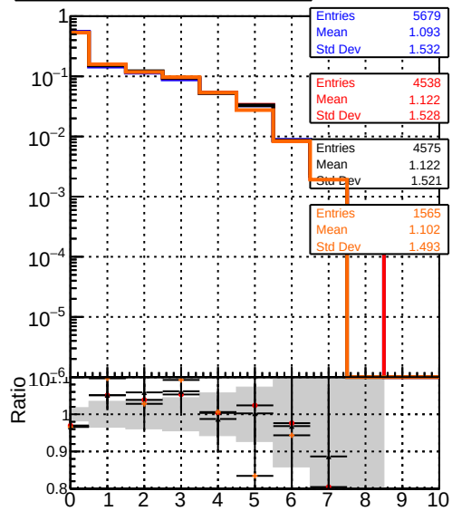
Legend: DQM_V0001_R000000001_Global_mkFit_baseline (blue line), DQM_V0001_R000000001_Global_mkFit_var (red line), DQM_V0001_R000000001_Global_mkFit_coreNoClean (black line), DQM_V0001_R000000001_Global_mkFit_icore50maxCand-45DUPremoval (orange line)
