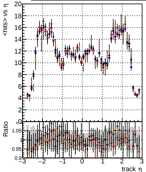
mean hits vs \eta Legend: DQM_V0001_R0000000001_Global_mkFit_baseline (blue line), DQM_V0001_R0000000001_Global_mkFit_var (red line), DQM_V0001_R0000000001_Global_mkFit_coreNoClean (black line), DQM_V0001_R0000000001_Global_mkFit_core50maxCand-45DUPremoval (orange line)
