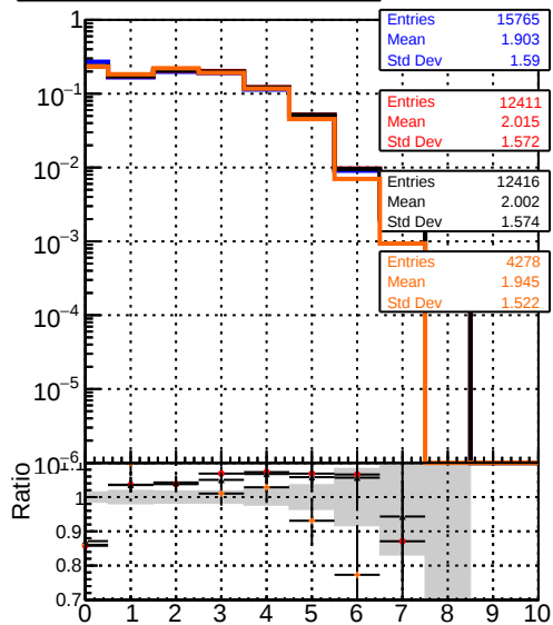
Legend: DQM_V0001_R000000001_Global_mkFit_baseline (blue), DQM_V0001_R000000001_Global_mkFit_var (red), DQM_V0001_R000000001_Global_mkFit_coreNoClean (black), DQM_V0001_R000000001_Global_mkFit_core50maxCand-45DUPremoval (orange) mean hits
