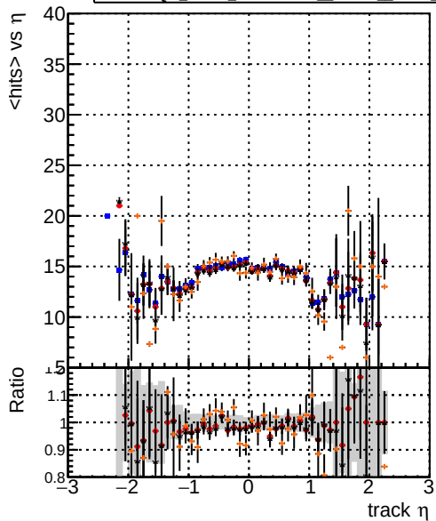
mean hits vs \eta Legend: DQM_V0001_R000000001_Global_mkFit_baseline (blue), DQM_V0001_R000000001_Global_mkFit_var (red), DQM_V0001_R000000001_Global_mkFit_coreNoClean (black), DQM_V0001_R000000001_Global_mkFit_core50maxCand-45DUPremoval (orange)
