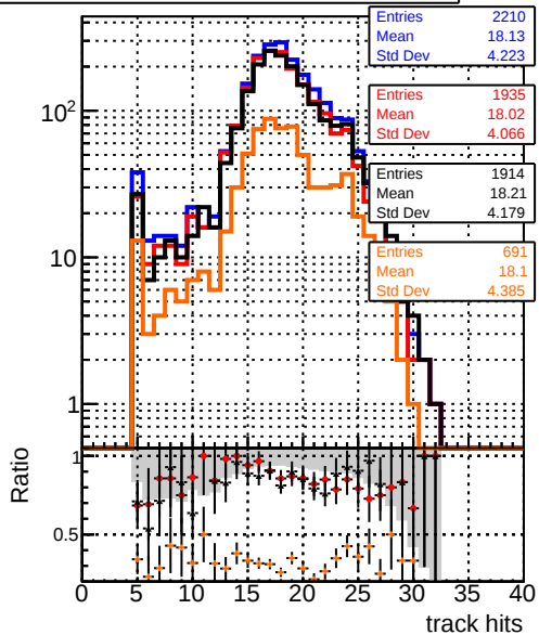
mean hits Legend: DQM_V0001_R000000001_Global_mkFit_baseline (blue line), DQM_V0001_R000000001_Global_mkFit_var (red line), DQM_V0001_R000000001_Global_mkFit_coreNoClean (black line), DQM_V0001_R000000001_Global_mkFit_core50maxCand-45DUPremoval (orange line)
