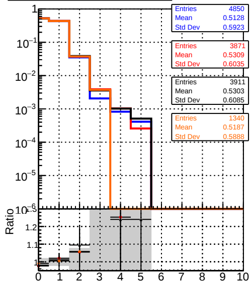
mean hits DQM_V0001_R000000001 Global mkFit baseline DQM_V0001_R000000001 Global mkFit var DQM_V0001_R000000001 Global mkFit jcoreNoClean DQM_V0001_R000000001 Global mkFit jcore50maxCand-45DUPremoval
