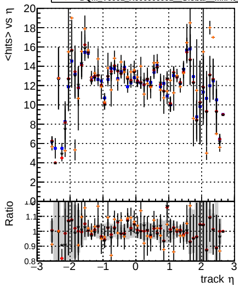
mean hits > \eta Legend: DQM_V0001_R000000001_Global_mkFit_baseline (blue), DQM_V0001_R000000001_Global_mkFit_var (red), DQM_V0001_R000000001_Global_mkFit_jcoreNoClean (black), DQM_V0001_R000000001_Global_mkFit_jcore50maxCand-45DUPremoval (orange)
