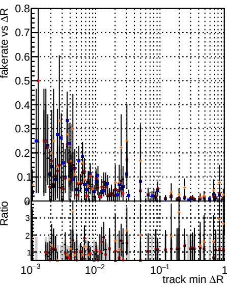
Fake rate vs \Delta R(\text{track, jet}) Legend: DQM V00001 R000000000001 Global mkFit baseline DQM V00001 R000000000001 Global mkFit var DQM V00001 R000000000001 Global mkFit coreNoClean DQM V00001 R000000000001 Global mkFit core50maxCand-45DUPremoval
