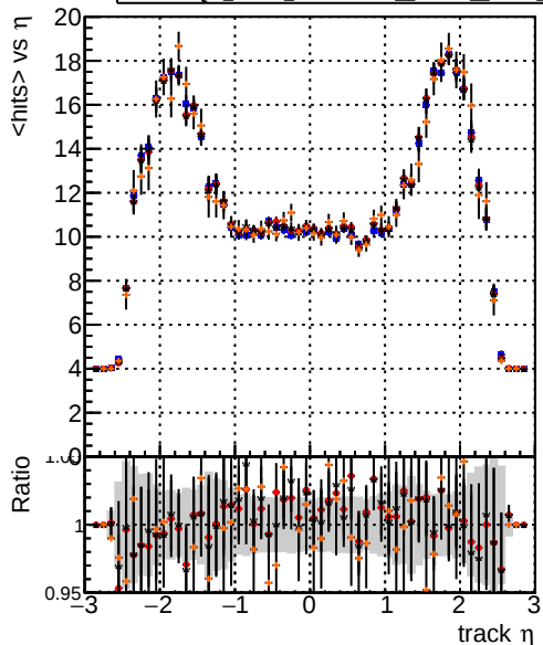
mean hit DQM_V0001_R000000001 Global mkFit baseline DQM_V0001_R000000001 Global mkFit var DQM_V0001_R000000001 Global mkFit jcoreNoClean DQM_V0001_R000000001 Global mkFit jcore50maxCand-45DUPremoval
