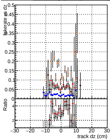
Fake rate vs dz Legend: BGM V0001 (blue) BGM V0001 (red) BGM V0001 (orange) Global (black) Global (grey) mkFit baseline mkFit var mkFit core50maxClean mkFit core50maxAnd45DUPremoval
