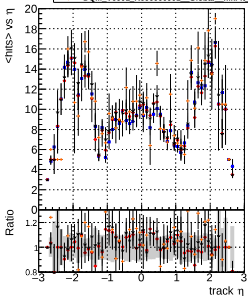
mean hit \eta DQM_V0001_R000000001 Global mkFit baseline DQM_V0001_R000000001 Global mkFit var DQM_V0001_R000000001 Global mkFit jcoreNoClean DQM_V0001_R000000001 Global mkFit jcore50maxCand-45DUPremoval
