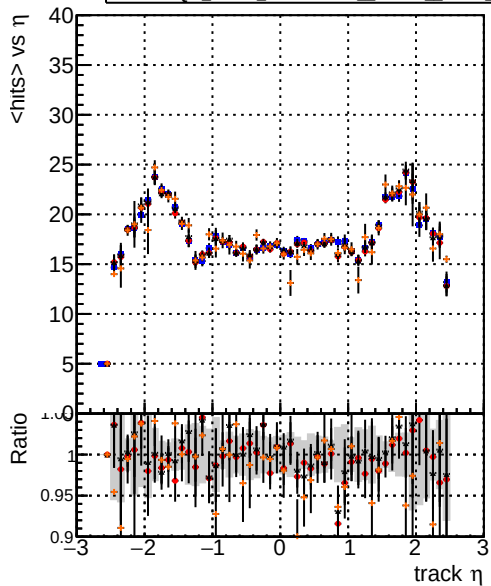
mean hit DQM_V0001_R000000001 Global mkFit baseline DQM_V0001_R000000001 Global mkFit var DQM_V0001_R000000001 Global mkFit jcoreNoClean DQM_V0001_R000000001 Global mkFit jcore50maxCand-45DUPremoval
