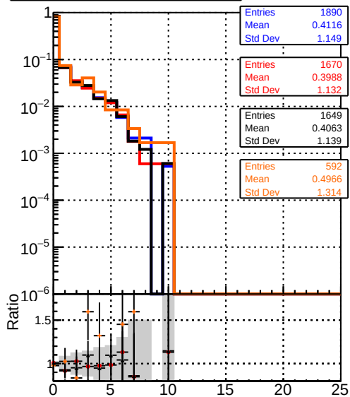
mean hit DQM_V0001_R000000001 Global mkFit baseline DQM_V0001_R000000001 Global mkFit var DQM_V0001_R000000001 Global mkFit jcoreNoClean DQM_V0001_R000000001 Global mkFit jcore50maxCand-45DUPremoval
