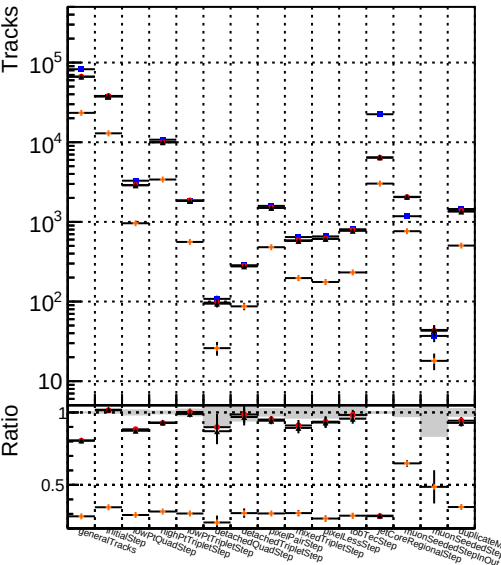
Number Model Configuration Method Baseline Var CoreNoClean Core50maxCand-45DUPremoval 1 DOM V0001 R0000000001 Global mkFit baseline 2 DOM V0001 R0000000001 Global mkFit var 3 DOM V0001 R0000000001 Global mkFit coreNoClean 4 DOM V0001 R0000000001 Global mkFit core50maxCand-45DUPremoval
