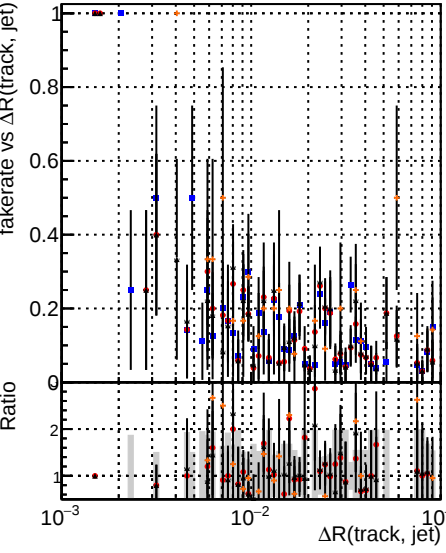
Fake rate vs \Delta R(\text{track, jet}) DQM V00001 R00000000001 Global mktFit baseline Core50maxCand-45DUPremoval
