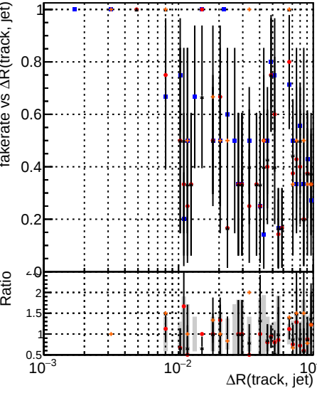
Fake rate vs \Delta R(\text{track, jet}) | Duplicates Rate vs \Delta R(\text{track, jet}) | Pileup rate vs \Delta R(\text{track, jet}) | Fake rate vs pu | Duplicates Rate vs pu | Pileup rate vs pu Legend: Global mkFit baseline, Global mkFit var, Global mkFit coreNoClean, Global mkFit core50maxCand-45DUPremoval
