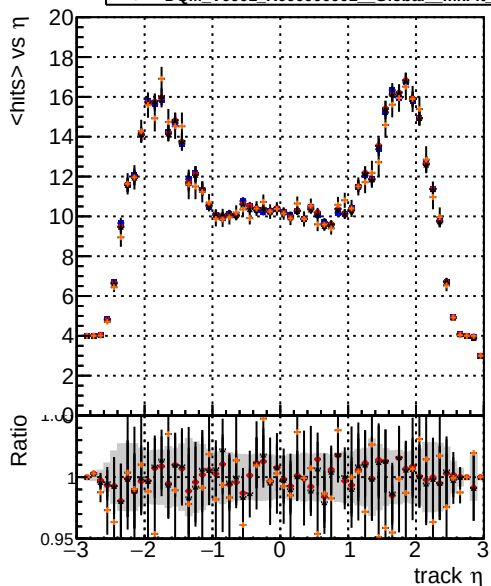
mean hits DQM_V0001_R000000001 Global mkFit baseline DQM_V0001_R000000001 Global mkFit var DQM_V0001_R000000001 Global mkFit jcoreNoClean DQM_V0001_R000000001 Global mkFit jcore50maxCand-45DUPremoval
