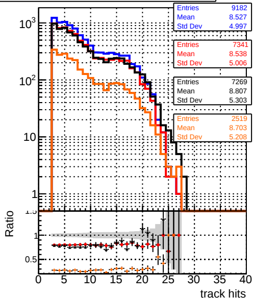
mean hits DQM_V0001_R000000001 Global mkFit baseline DQM_V0001_R000000001 Global mkFit var DQM_V0001_R000000001 Global mkFit jcoreNoClean DQM_V0001_R000000001 Global mkFit jcore50maxCand-45DUPremoval
