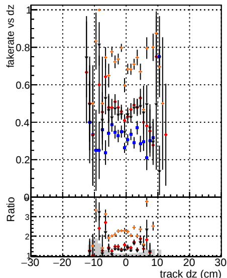
Fake rate vs dz Legend: DQM V0001 Global fit baseline Global fit var Global fit core50max Global fit Clean Global fit Clean and 45DUPremoval
