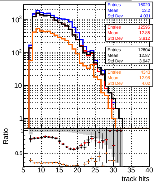
Legend: DQM_V0001_R000000001 Global mkFit baseline, DQM_V0001_R000000001 Global mkFit var, DQM_V0001_R000000001 Global mkFit jcoreNoClean, DQM_V0001_R000000001 Global mkFit jcore50maxCand-45DUPremoval
