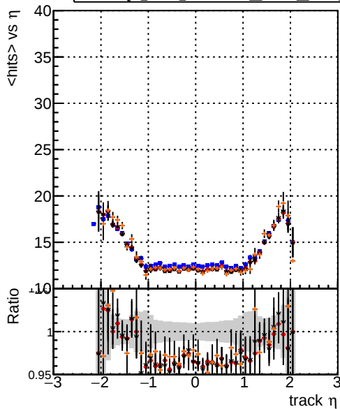
Legend: DQM_V0001_R000000001 Global mkFit baseline, DQM_V0001_R000000001 Global mkFit var, DQM_V0001_R000000001 Global mkFit jcoreNoClean, DQM_V0001_R000000001 Global mkFit jcore50maxCand-45DUPremoval
