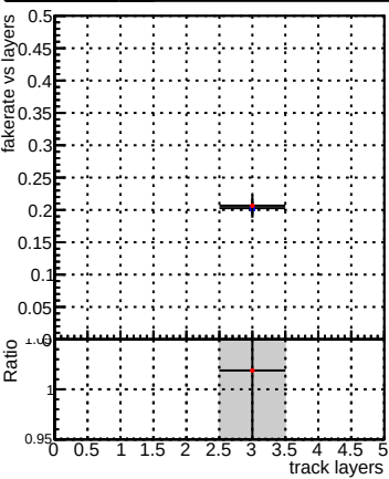
Fake rate vs layers
