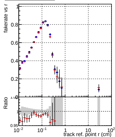
■ DQM_V0001_R000000001_Global_mkFit_baseline ● DQM_V0001_R000000001_Global_mkFit_var
