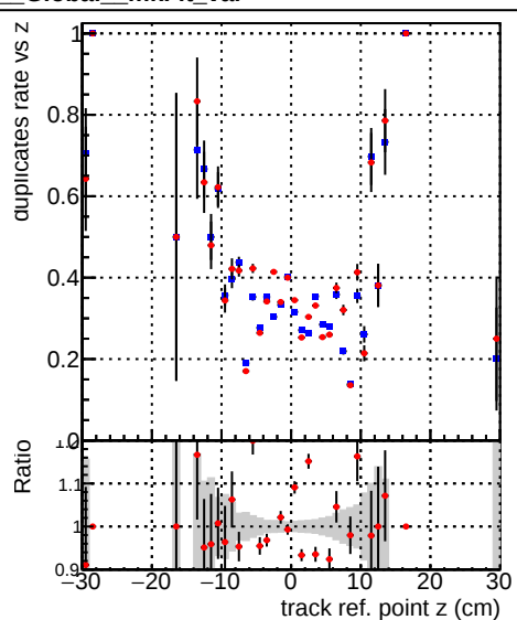
■ DQM_V0001_R000000001_Global_mkFit_baseline ● DQM_V0001_R000000001_Global_mkFit_var
