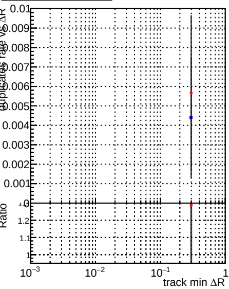
Legend: DQM_V0001_R000000001_Global_mkFit_baseline (blue squares), DQM_V0001_R000000001_Global_mkFit_var (red circles)
