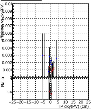
Efficiency vs Dxy(PV) Legend: DQM_V0001_R000000001_Global_mkFit_baseline DQM_V0001_R000000001_Global_mkFit_var DQM_V0001_R000000001_Global_mkFit_jcoreNoClean
