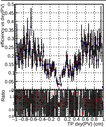
Efficiency vs Dxy(PV) plot showing efficiency and ratio vs TP dxy(PV) (cm). The legend indicates three data series: DQM_V0001_R000000001_Global_mkFit_baseline (blue squares), DQM_V0001_R000000001_Global_mkFit_var (red circles), and DQM_V0001_R000000001_Global_mkFit_jcoreNoClean (black circles).
