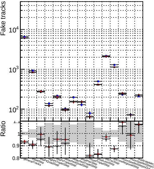
Number DQM_V0001_R0000000001_Global_mkFit_baseline DQM_V0001_R0000000001_Global_mkFit_var DQM_V0001_R0000000001_Global_mkFit_jcoreNoClean
