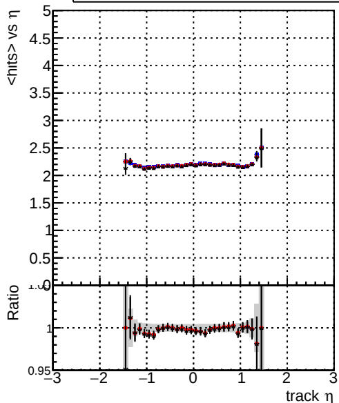
mean hit — DQM_V0001_R000000001_Global_mkFit_baseline — DQM_V0001_R000000001_Global_mkFit_var — DQM_V0001_R000000001_Global_mkFit_coreNoClean
