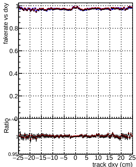
Legend for Fake rate vs dxy, Duplicates Rate vs Dxy, and Pileup rate vs dxy: DOM V0001 R0000000001 Global mkFit baseline DOM V0001 R0000000001 Global mkFit var DOM V0001 R0000000001 Global mkFit icoreNoClean
