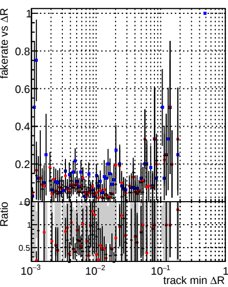
Fake rate vs \Delta R(\text{track, jet}) Legend: DQM_V0001_R000000001 Global mkFit_baseline DQM_V0001_R000000001 Global mkFit_var DQM_V0001_R000000001 Global mkFit_jcoreNoClean
