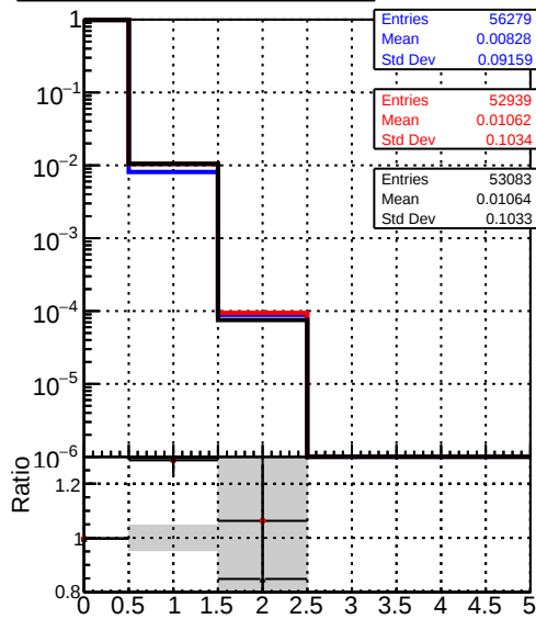
mean hits vs \eta — DQM_V0001_R000000001_Global_mkFit_baseline — DQM_V0001_R000000001_Global_mkFit_var — DQM_V0001_R000000001_Global_mkFit_coreNoClean
