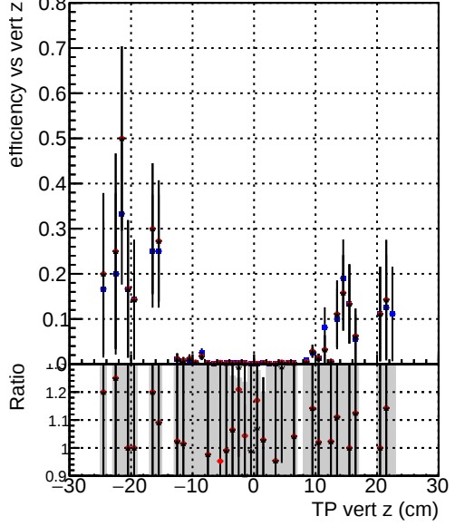
Efficiency vs vert z —●— DQM_V0001_R000000001_Global_mkFit_baseline —●— DQM_V0001_R000000001_Global_mkFit_var —●— DQM_V0001_R000000001_Global_mkFit_coreNoClean
