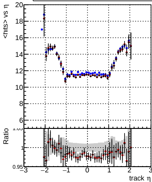
mean hit — DQM_V0001_R000000001_Global_mkFit_baseline — DQM_V0001_R000000001_Global_mkFit_var — DQM_V0001_R000000001_Global_mkFit_coreNoClean
