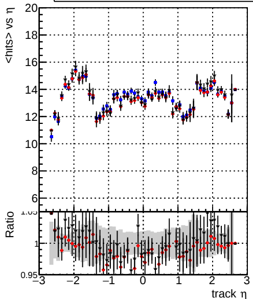
mean hit — DQM_V0001_R000000001_Global_mkFit_baseline — DQM_V0001_R000000001_Global_mkFit_var — DQM_V0001_R000000001_Global_mkFit_coreNoClean
