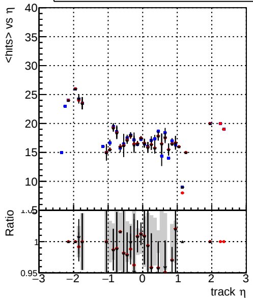
— DQM_V0001_R000000001_Global_mkFit_baseline — DQM_V0001_R000000001_Global_mkFit_var — DQM_V0001_R000000001_Global_mkFit_coreNoClean
