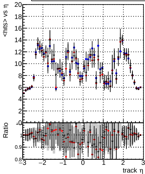
— DQM_V0001_R000000001_Global_mkFit_baseline — DQM_V0001_R000000001_Global_mkFit_var — DQM_V0001_R000000001_Global_mkFit_coreNoClean
