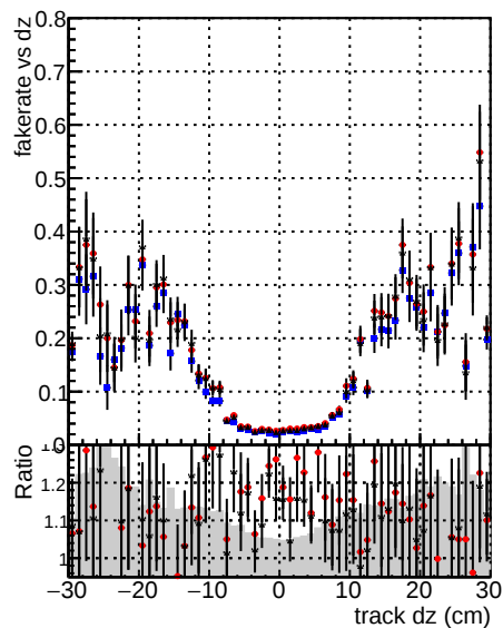
DOM V0001 R0000000001 Global mkFit baseline DOM V0001 R0000000001 Global mkFit var DOM V0001 R0000000001 Global mkFit coreNoClean
