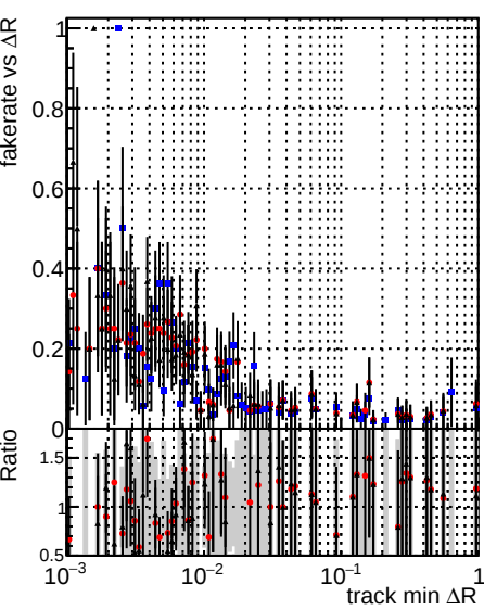
Legend: DQM_V0001_R0000000001 Global mkFit_baseline, DQM_V0001_R0000000001 Global mkFit_var, DQM_V0001_R0000000001 Global mkFit_jcoreNoClean
