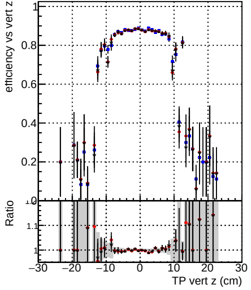
Efficiency vs. TP vert z —●— DQM_V0001_R0000000001_Global_mkFit_baseline —●— DQM_V0001_R0000000001_Global_mkFit_var —●— DQM_V0001_R0000000001_Global_mkFit_coreNoClean
