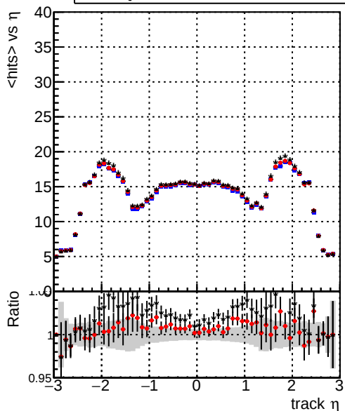
mean hits — DQM_V0001_R000000001_Global_mkFit_baseline — DQM_V0001_R000000001_Global_mkFit_var — DQM_V0001_R000000001_Global_mkFit_coreNoClean
