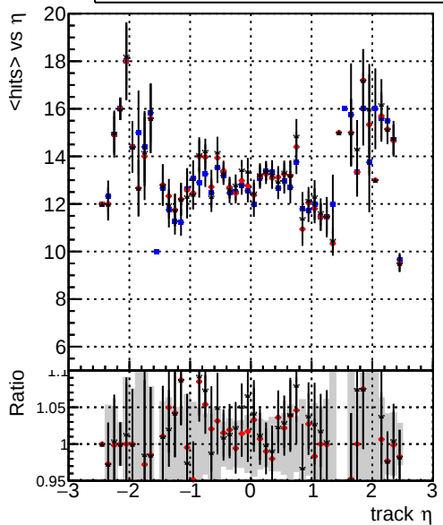
DQM_V0001_R000000001_Global_mkFit_baseline DQM_V0001_R000000001_Global_mkFit_var DQM_V0001_R000000001_Global_mkFit_coreNoClean mean hit
