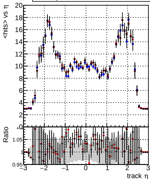
— DQM_V0001_R000000001_Global_mkFit_baseline — DQM_V0001_R000000001_Global_mkFit_var — DQM_V0001_R000000001_Global_mkFit_jcoreNoClean
